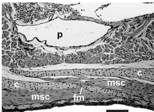
Fig. 9. Larva of Salamandrella keyserlingii , stage 52. Fragment of transverse section in the pectoral girdle region. c , Coracoid part; fm , “muscle” foramen; msc , m. supracoracoideus ; p , pericardial cavity. Scale bar is 150 \mu m.
